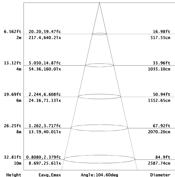
Lux-Distance Curve
